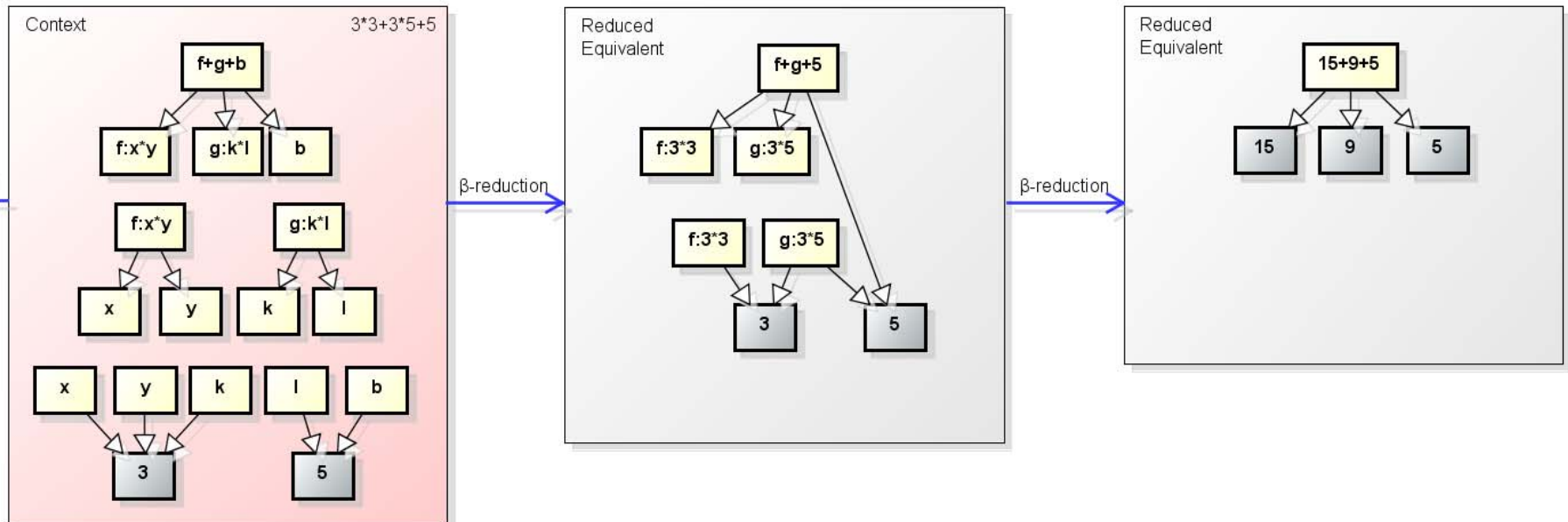
Different types of Factorization
